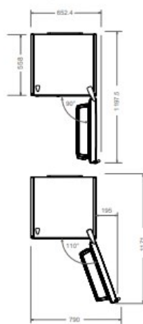
TOP VIEW
